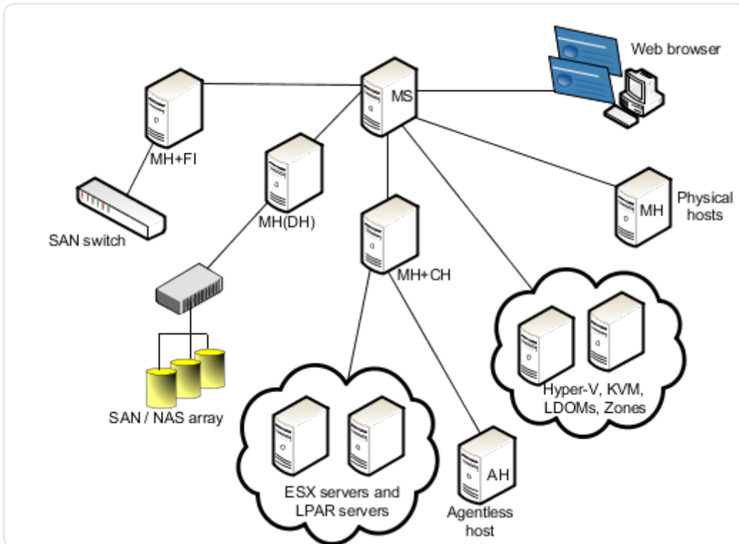
Figure: Veritas InfoScale Operations Manager components and discovery (virtualization servers and virtual machines)
